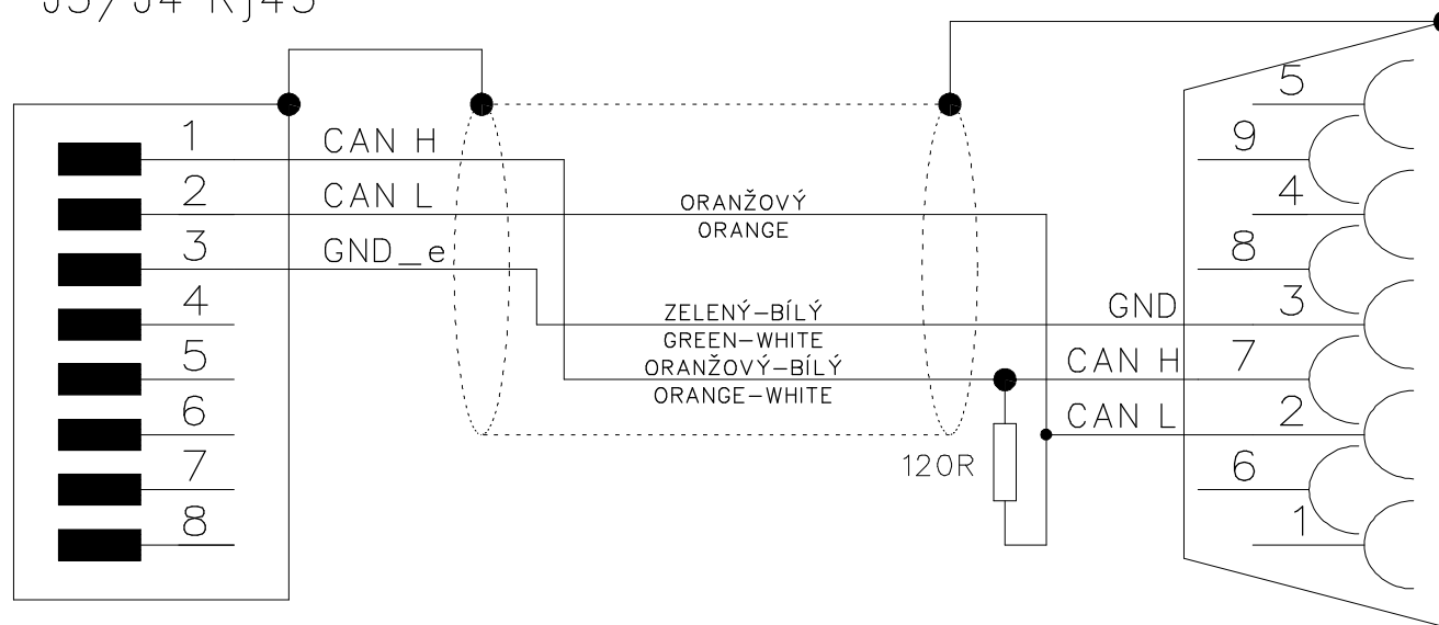
CAN INTERFACE TG_I/O_40/24/4/4 J3/J4 Rj45
