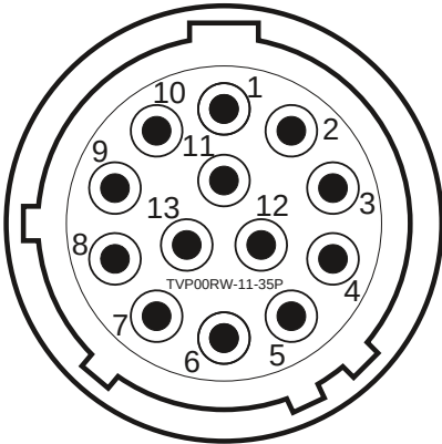
Connector 2 (267)
