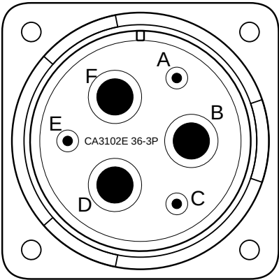
Connector 1 (454)
